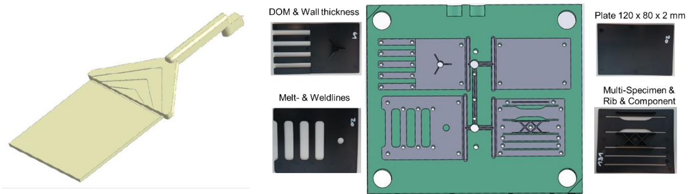
Fig.5: Injection molding: left – used mold in [7], right – used mold for failure evaluation and validation [8]
